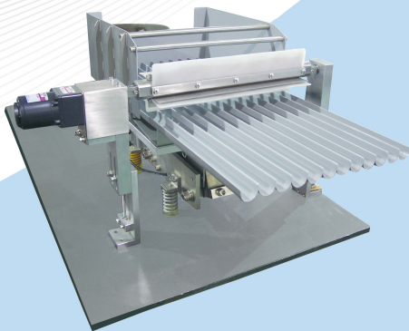
Meat ball feeding system (12 lanes)
