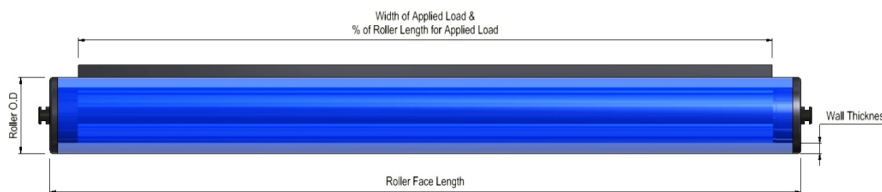
Conveyor Idler Load Profile - Aluminium & Steel
