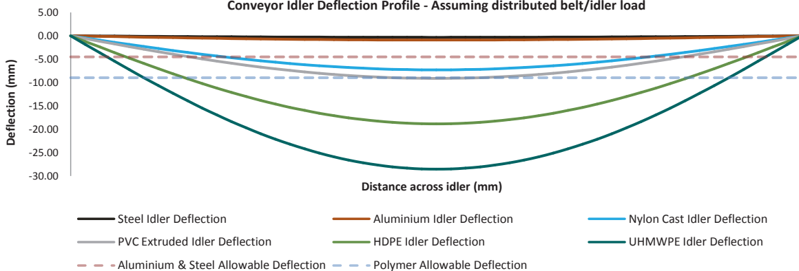
Conveyor Idler Deflection Profile - Assuming distributed belt/idler load
